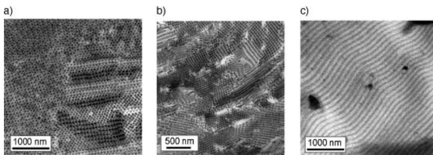
Figure 10. Electron micrographs of a cubic (a), hexagonal (b), and lamellar (c) superlattice of block copolymers in lyotropic liquid crystalline phases. The structure of the lyotropic phases was fixed by \gamma irradiation. [50, 95]
