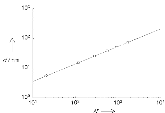
Figure 12. Long period d as a function of the degree of polymerization N of PB-PEO ( \square ) and nonionic surfactants ( \circ ). [50] The periodic length of the nanostructure can be specifically adjusted over the whole mesoscopic range (1–100 nm) by the degree of polymerization.
