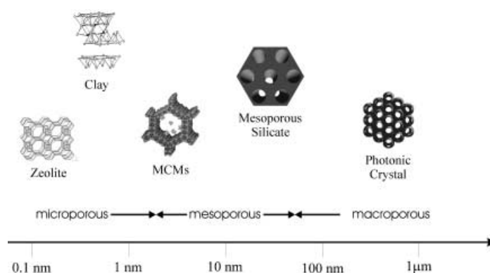
Figure 23. Typical length scales of three-dimensional porous structures.
